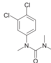
Diuron Structure
