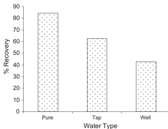
Figure 4 Effect of water type on diuron preconcentration at 100 \mu\text{g/L} .
