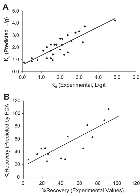
Figure 3 Prediction of K_d (A) and %recovery (B) using PCA.
