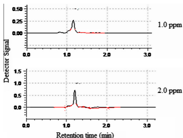
Figure 1 Chromatograms of diuron at two different concentrations.
