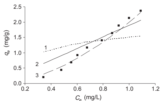
Figure 2 Adsorption isotherm of diuron at 25 °C (mass of HDS: 40 mg, volume of solution 50 mL, pH 7, and shaking time 7 days). (1) Longmuir's model, (2) Henry's model, and (3) Ferundlich's model.
